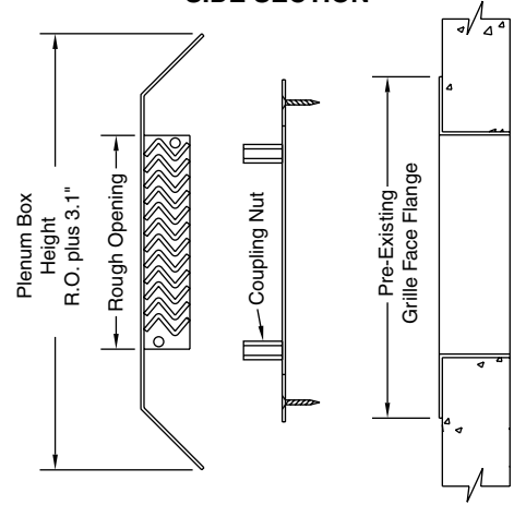
SIDE SECTION
