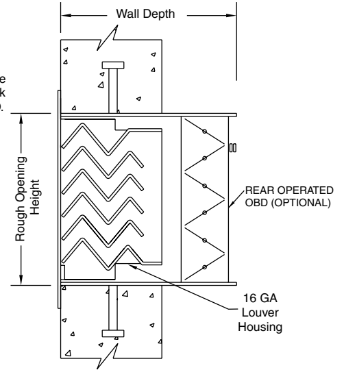
SIDE SECTION
