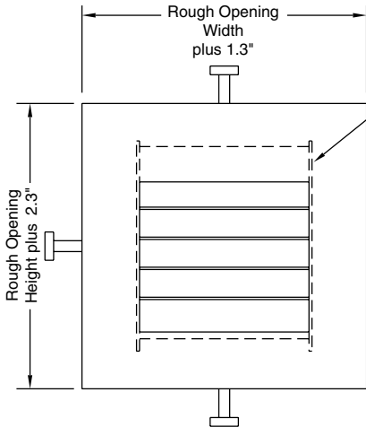
FRONT SECTION
