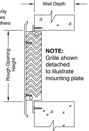
SIDE SECTION
