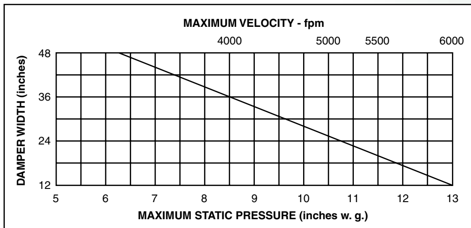
GRAPH 17: MAXIMUM STATIC PRESSURE/VELOCITY
