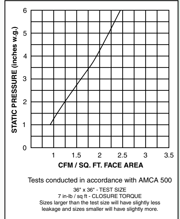
GRAPH 16: LEAKAGE
