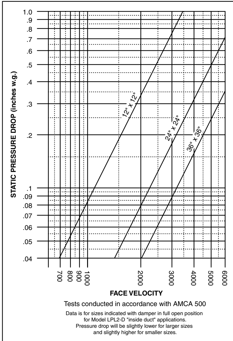
GRAPH 15: AIR PRESSURE DROP
