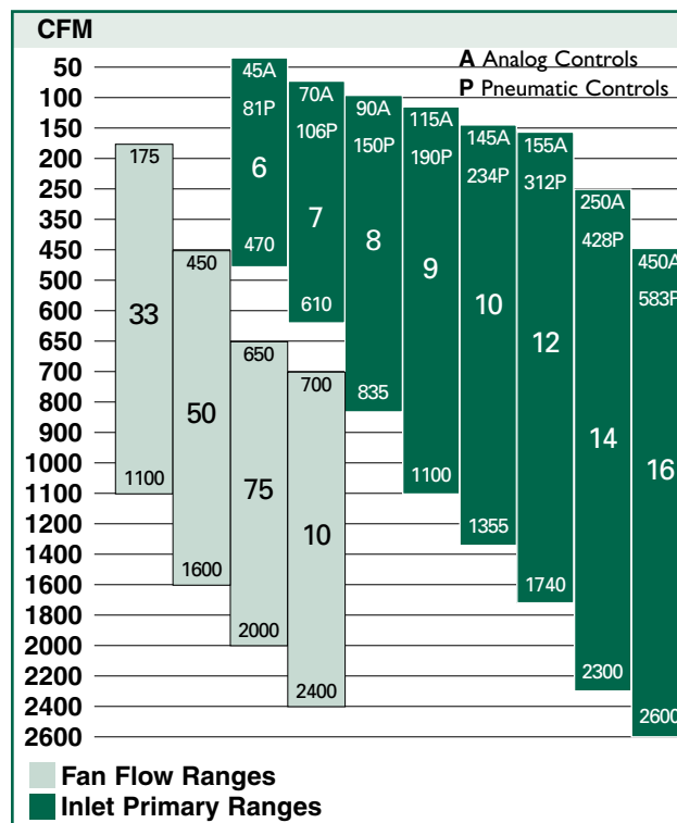
Chart 2: Unit Flow Ranges
