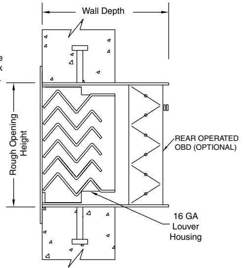
SIDE SECTION
